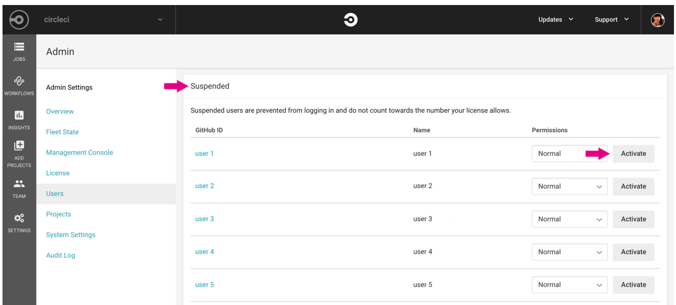
Figure 17. Reactivate Existing Users
