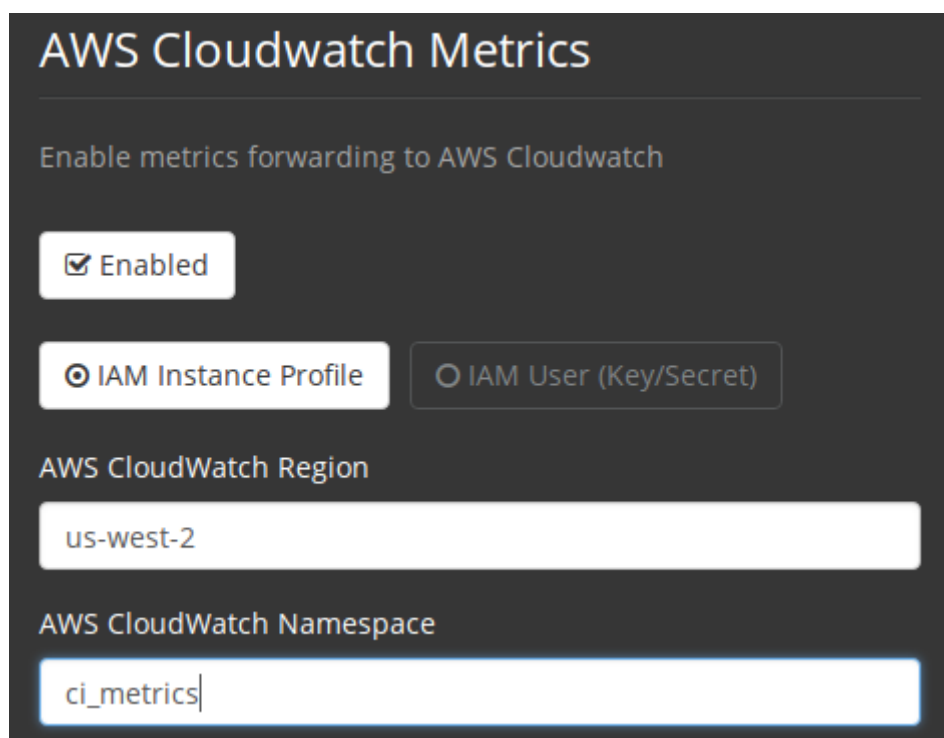
Figure 5. CloudWatch Region and Namespace
