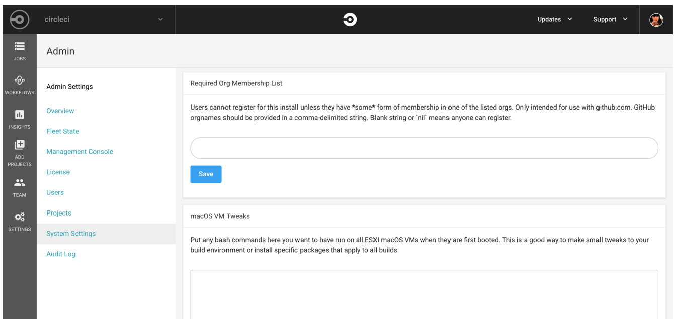
Figure 20. Organization Membership
