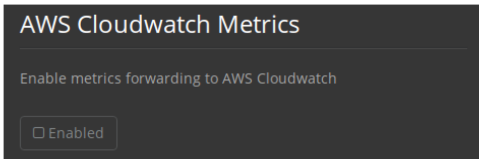
Figure 4. Enable Cloudwatch
