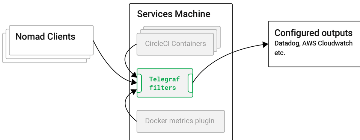
Figure 3. Metrics
